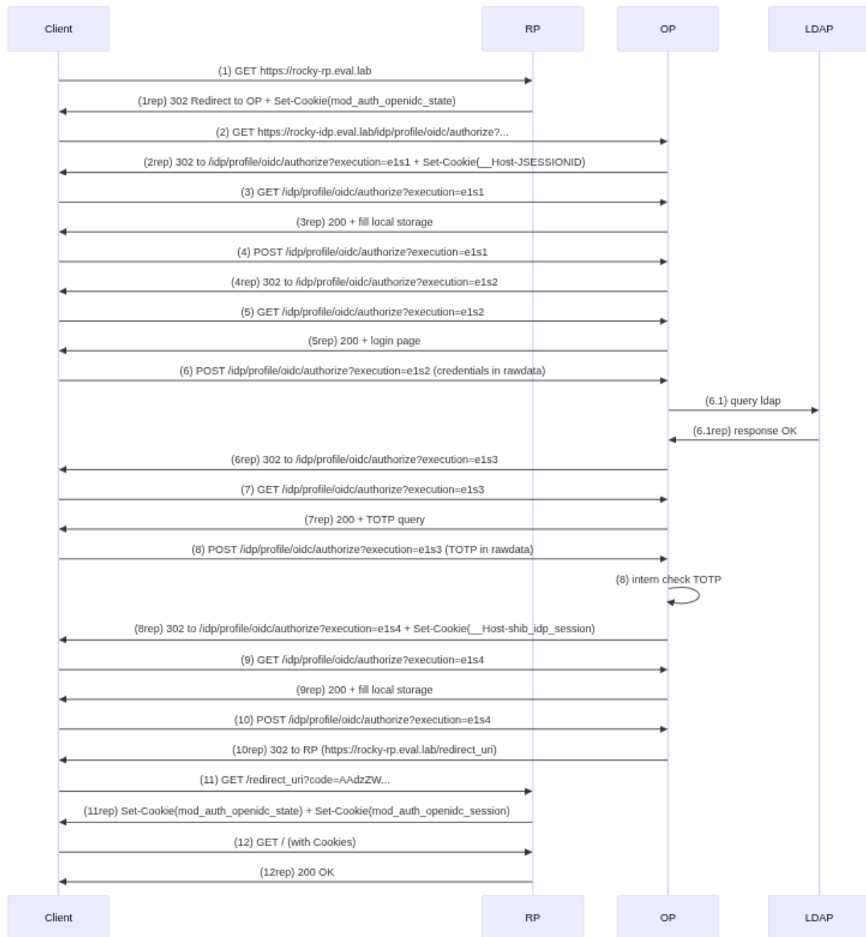
Figure 11 - OIDC with MFA authentication flow
