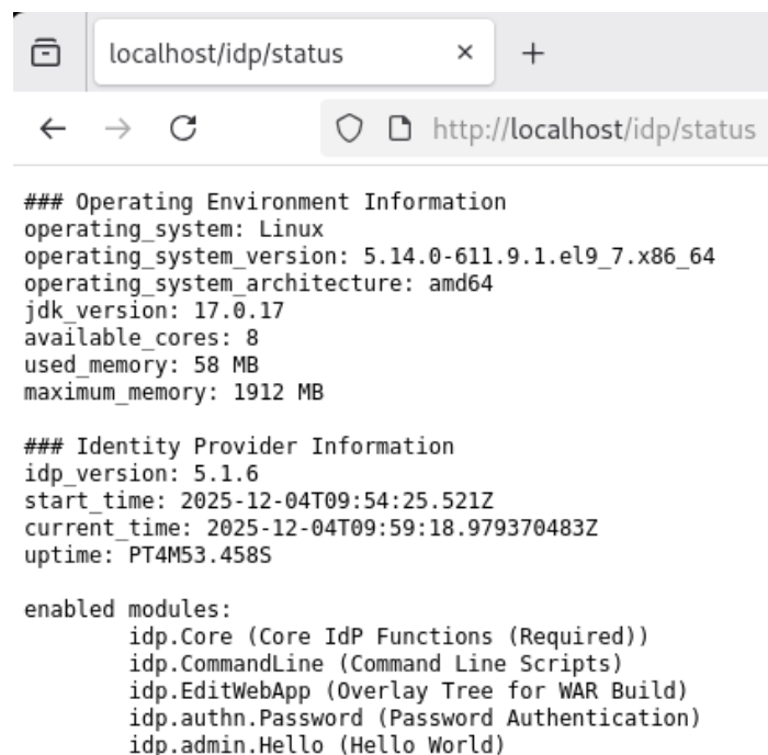
Figure 1 - Version identification of Shibboleth IdP
