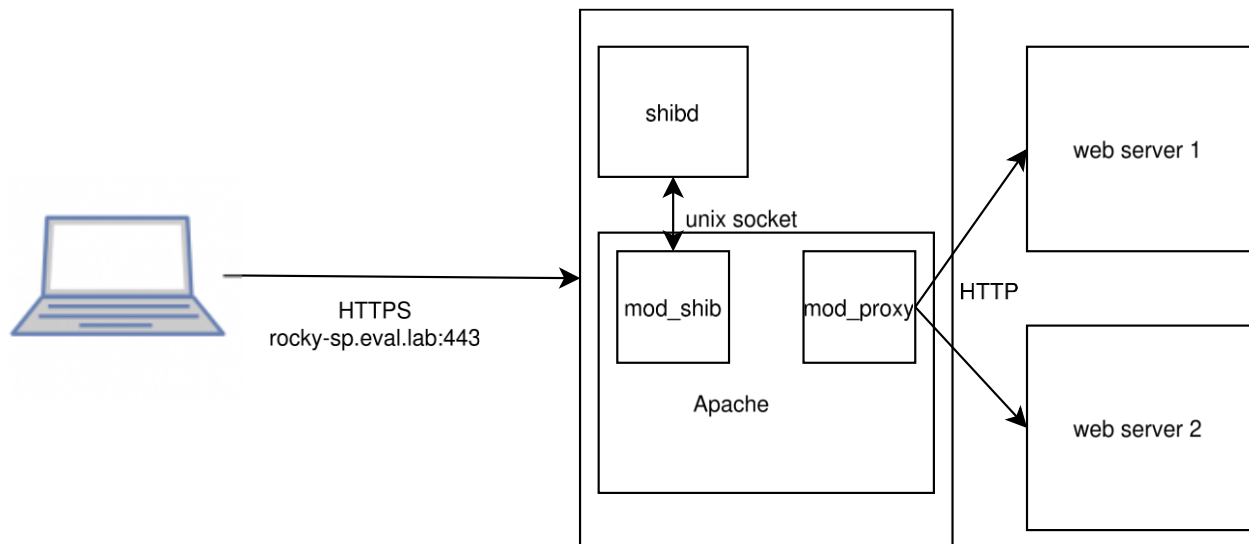
Figure 4 - Internal SP configuration
