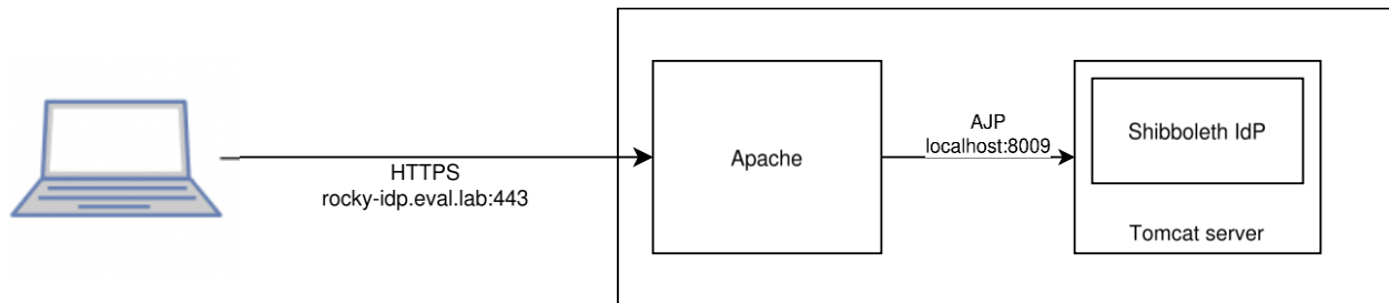
Figure 3 - Internal IdP configuration
