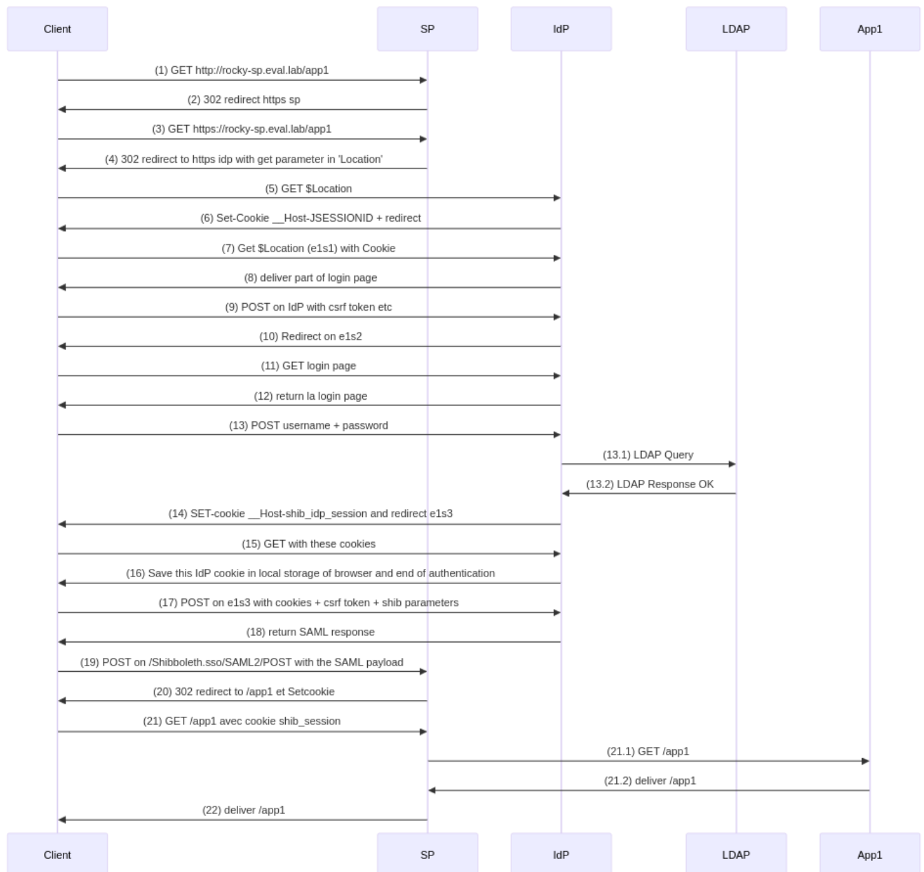
Figure 10 - Authentication Request Protocol
